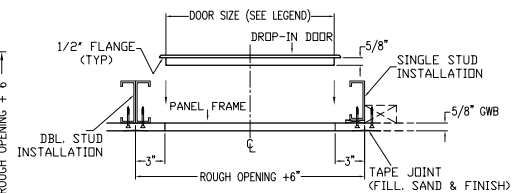
Drop-in Access Panel - Side View (Single/Double stud installation)
