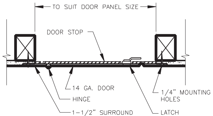
SECTION DETAIL
