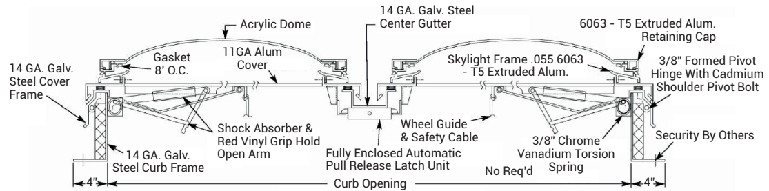
SECTION A - A SMOKE HATCH
