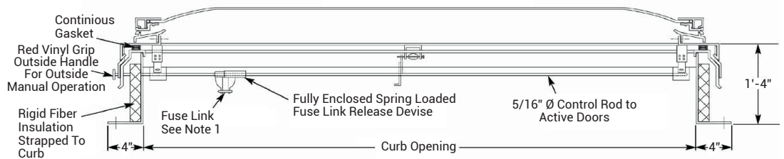
SECTION A - A SMOKE HATCH
