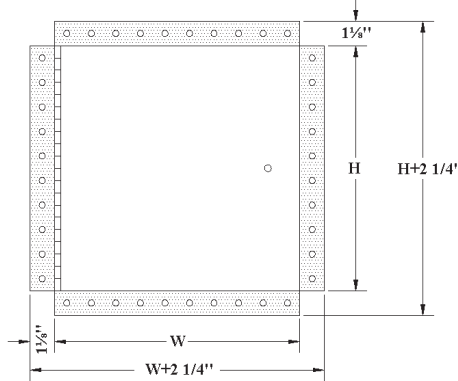
Rough wall opening is door size + 1/4" or + 6mm
