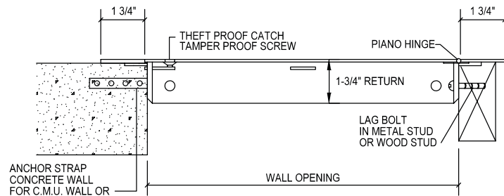
SECTION DETAIL
