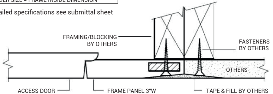
Drop-In Door Models
