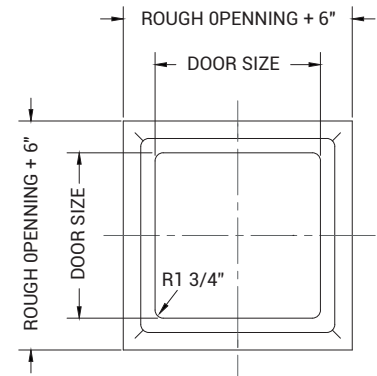
DROP-IN ACCESS PANEL - TYPE PANEL ELEVATIONS
