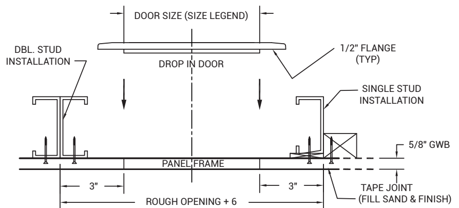
ACCESS PANEL - SIDE VIEW (SINGLE/DOUBLE STUD INSTALLATION)
