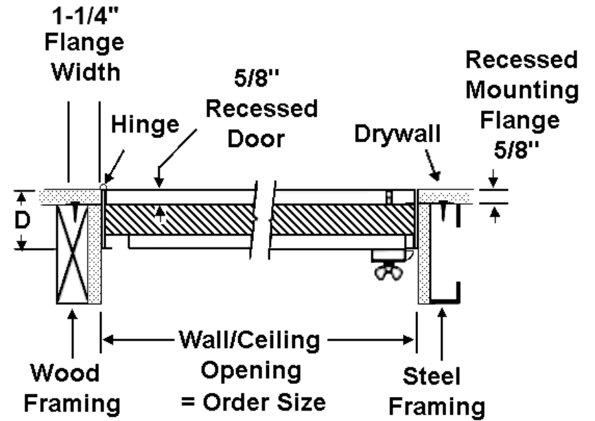
TYPICAL FRAMING OF ACCESS PANEL
