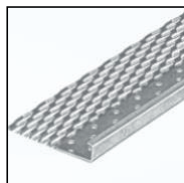
Metal lath with 3/4" deep plaster stop.
