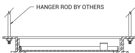
INSTALLATION DETAIL
