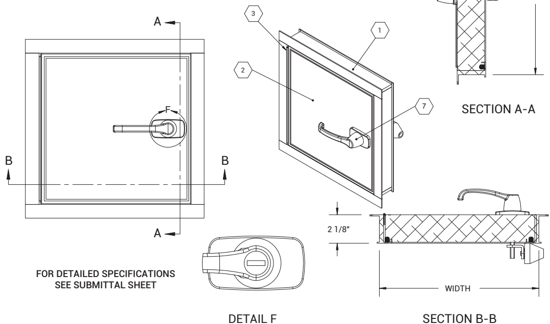
DETAIL F
