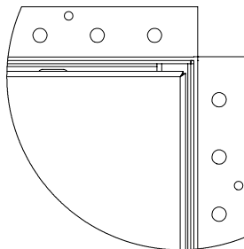
DETAIL D DRYWALL BEAD DETAIL SCALE 1 : 4
