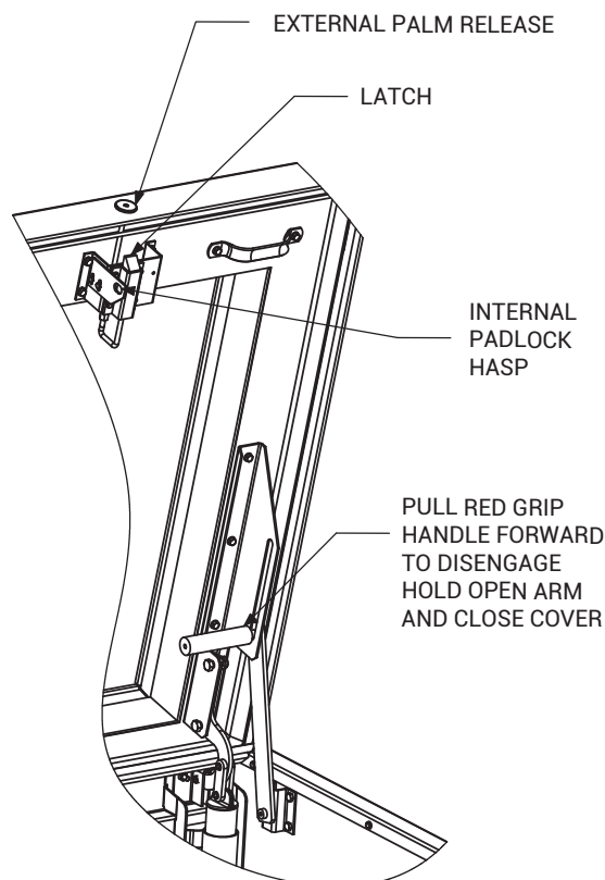
HARDWARE DETAILS
