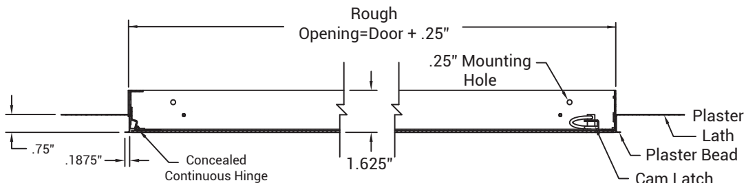
CUT-THRU SECTION NOT TO SCALE
