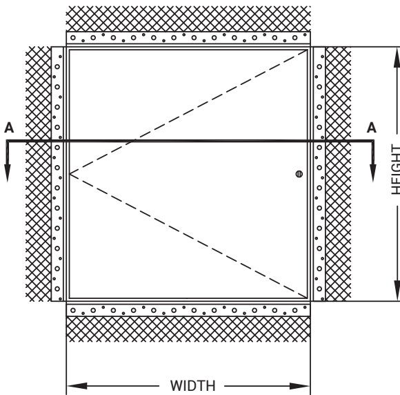
FRONT ELEVATION NOT TO SCALE
