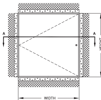
FRONT ELEVATION NOT TO SCALE
