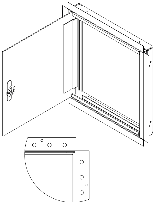
DETAIL D DRYWALL BEAD DETAIL SCALE 1 : 4
