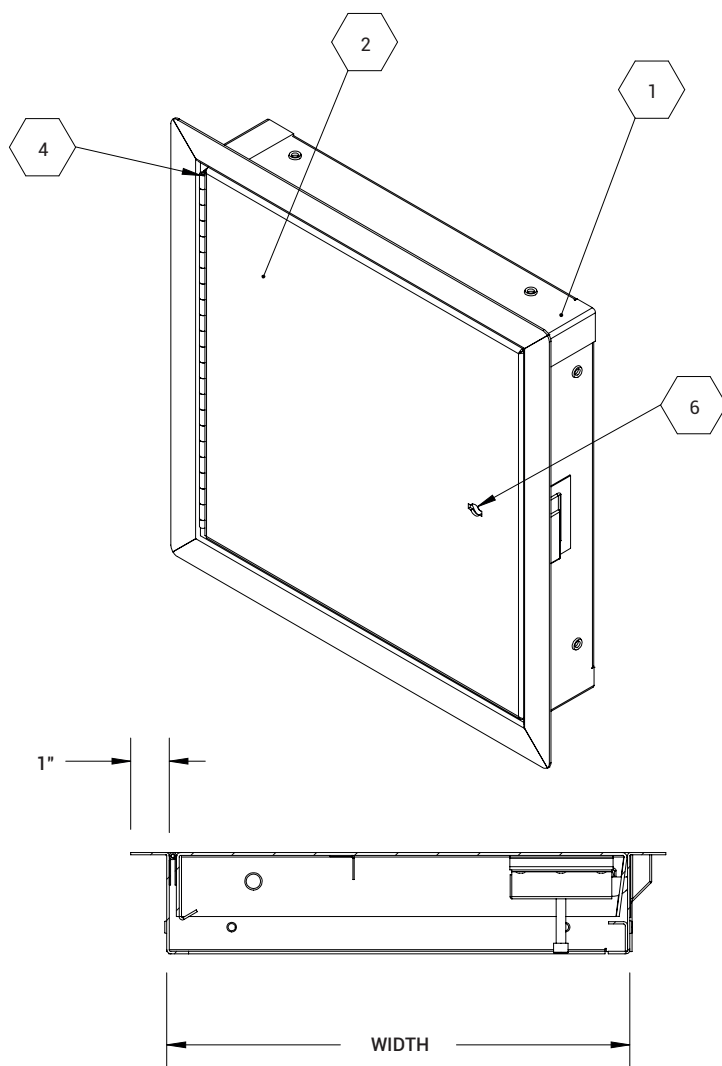
SECTION B-B
