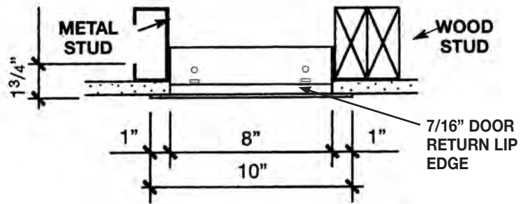
SECTION DETAIL
