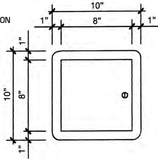
SECTION DETAIL
