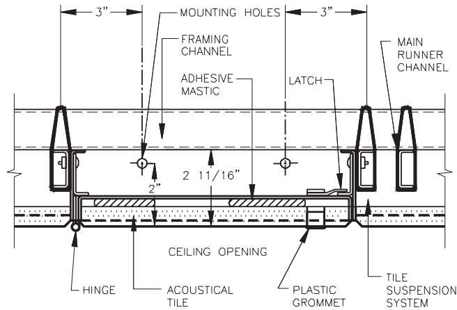
SECTION DETAIL
