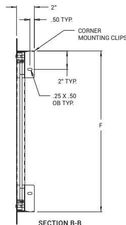
SECTION B-B
