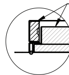
DETAIL A SCALE 1 : 6
